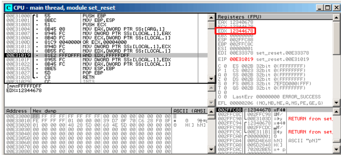
Figure 1.96: OllyDbg: value has been reloaded into EDX
