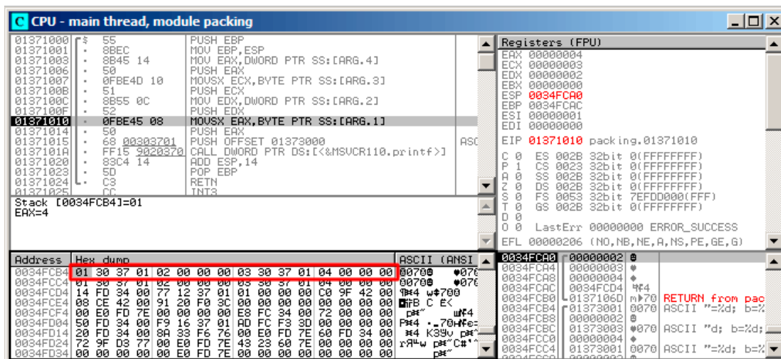
Figure 1.105: OllyDbg: Before printf() execution
