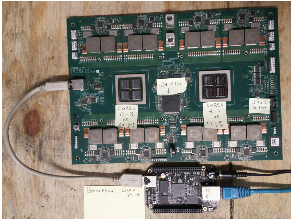
Figure 8.14: Board
