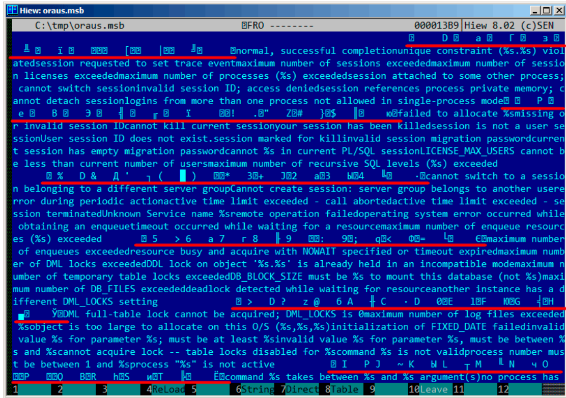
Figure 9.27: HiView: first block
